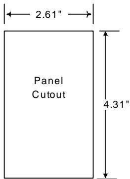
Figure 1: CT6000 Dimensions
