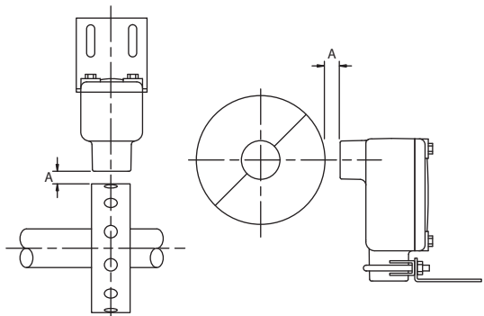
Figure 5: Explosion proof 907 Sensor and Pulser Wrap
