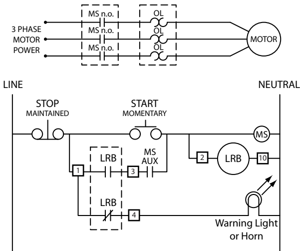
Figure 7: Typical Wiring Diagram
