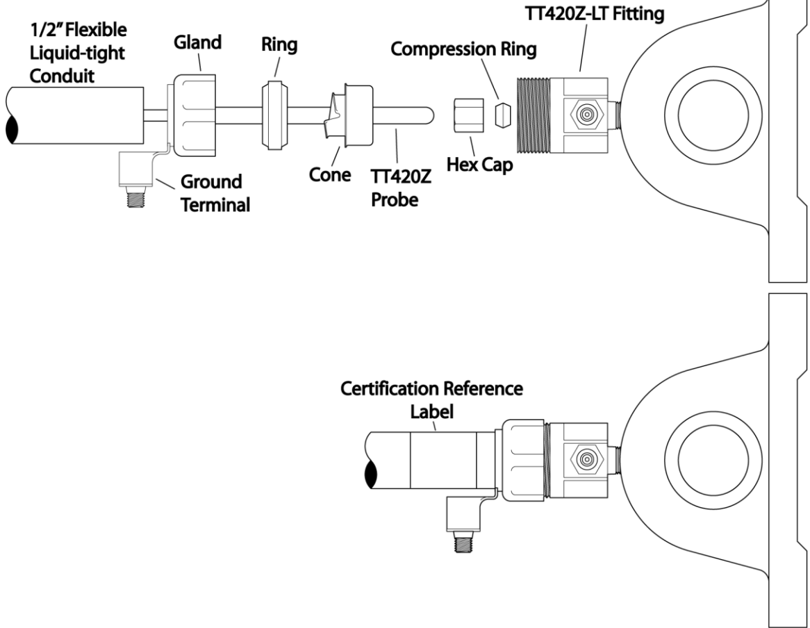
TT420Z-LT (1/2 in) installation
