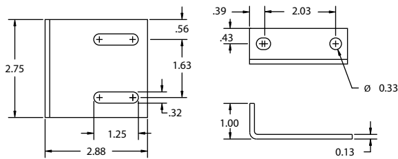
Explosion proof 907 Sensor Bracket
